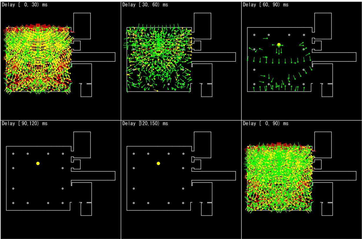
Figure 2: The case when the shape of ceiling is optimized.
