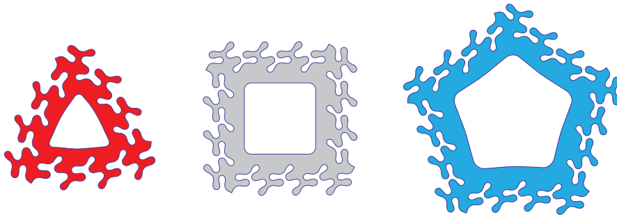
Figure 9: Improved Zippergons
