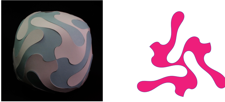
Figure 6: Octahedral sphere II
