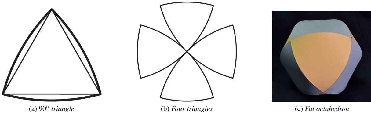
Figure 3: Fat octahedron
